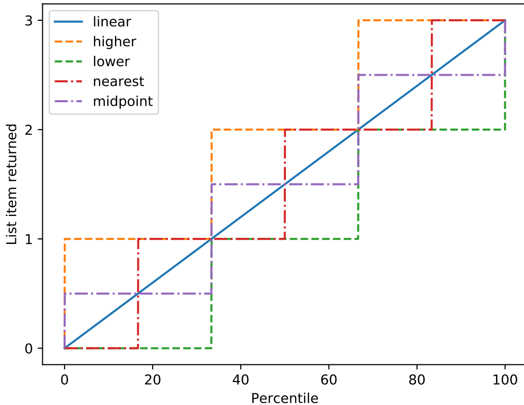
Interpolation methods for list: [0 1 2 3]
